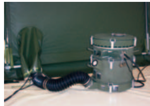
NBC-Filter System
